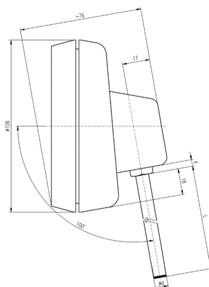
Angular thermometer
