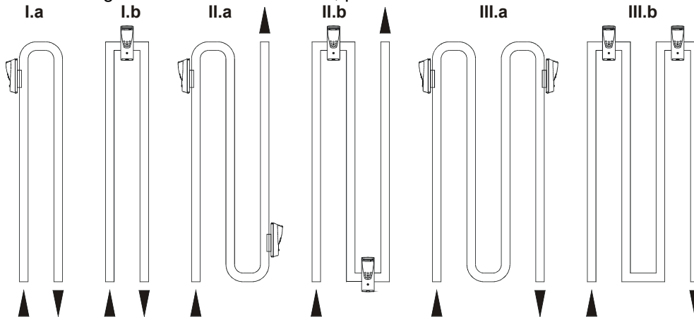
Illustration 12: E-ITN 30 location on vertical tubular radiators
