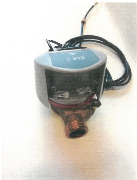
Picture 2: Sealing of compact thermal energy meters type Elf2, on side view, placement of serial number:
