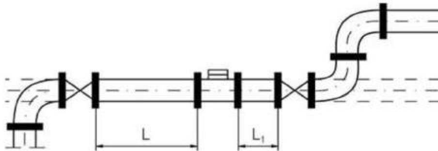
Picture 5: Water meter installation
