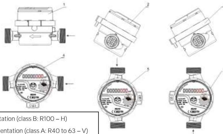
Picture 6: Sample permitted installation positions
