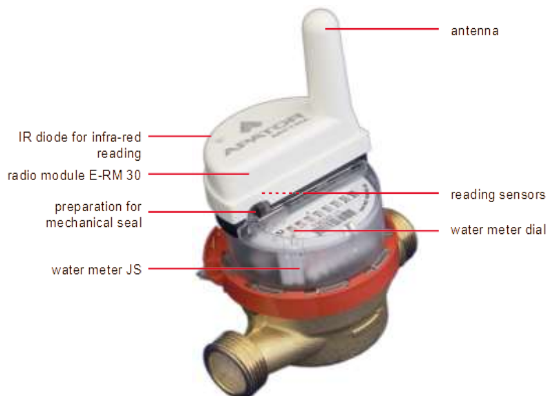
Picture 1: radio module E-RM 30 with water meter JS
